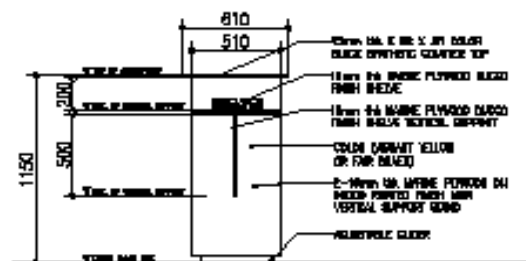
WRITING DECK SECTION THRU "A" SCALE: 1:20 METERS
