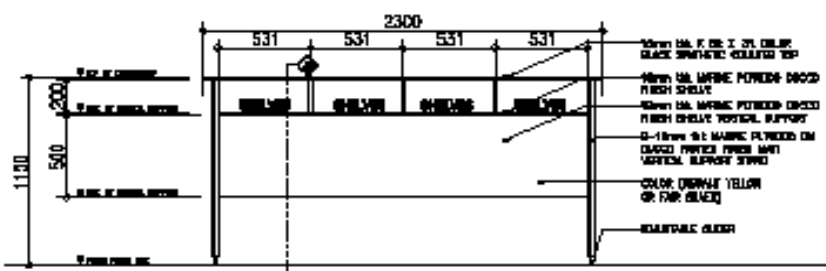
WRITING DECK FRONT ELEVATION SCALE: 1:20 METERS
