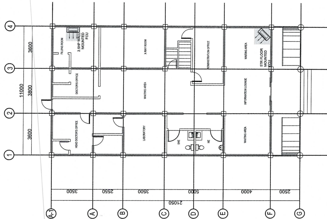
GROUND FLOOR PE BUILDING
